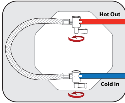
Water Heater Bypass Valves (Bypass Position Shown)
